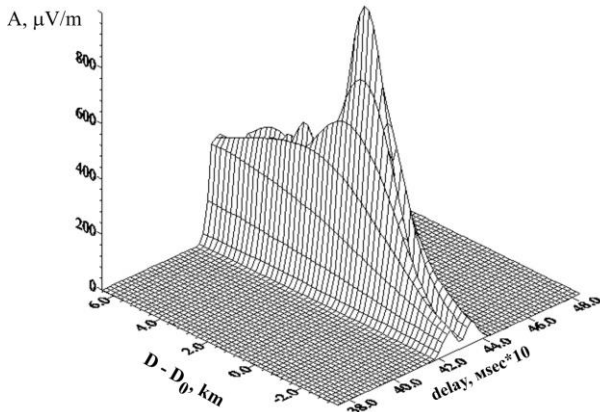
Figure 5. Range-time distribution of the signal envelope near the skip zone border for medium-wet soil
