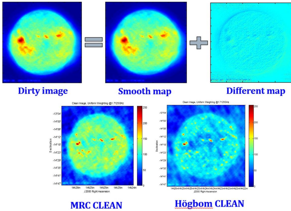
Figure 7. Simulated dirty image and restored images from MRC and Högbom CLEAN
