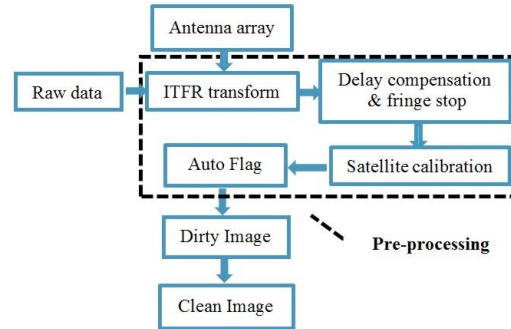
Figure 2. Imaging pipeline of MUSER
