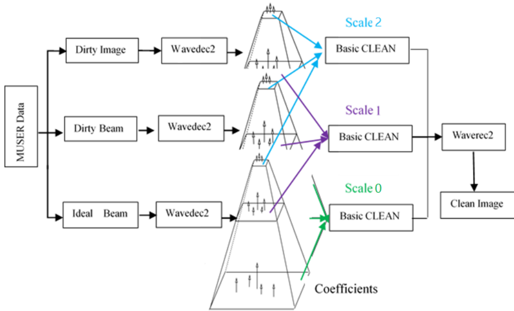
Figure 5. Framework of the Wavelet CLEAN
