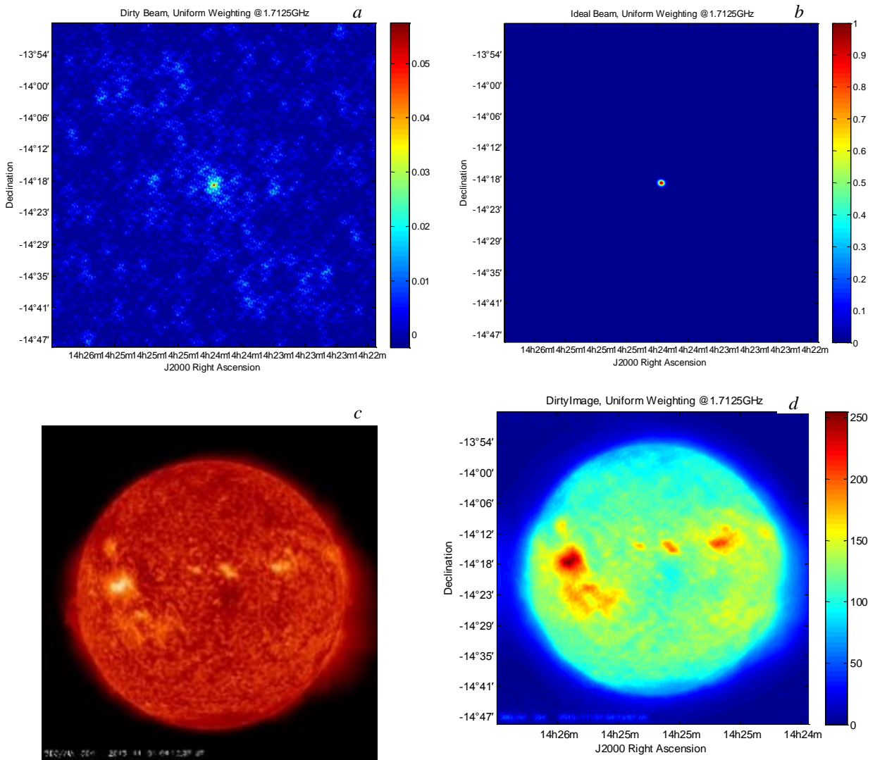
Figure 6. Simulated image on November 1, 2015: dirty beam from MUSER (a); clean beam from MUSER (b); AIA304 image (simulated ideal image) (c); simulated dirty image (d)
